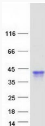
Coomassie blue staining of purified OBP2B protein.
