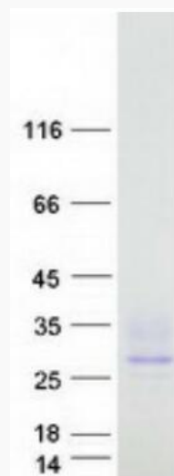
Coomassie blue staining of purified SHISAL2B protein.
