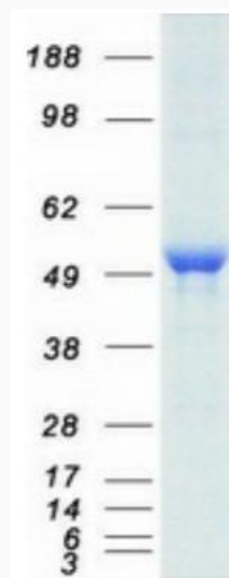
Coomassie blue staining of purified GCK protein.
