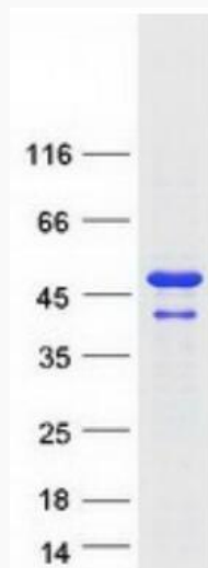
Coomassie blue staining of purified DDRGK1 protein.
