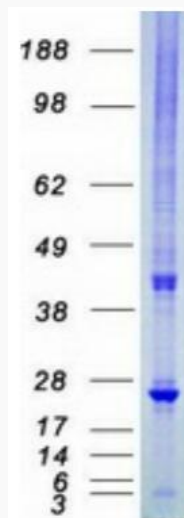
Coomassie blue staining of purified HSPB8 protein.
