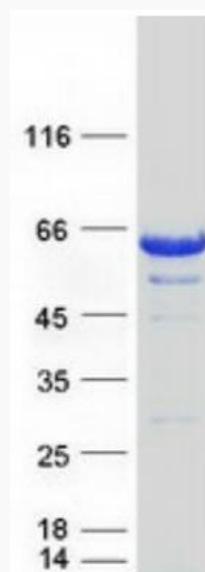
Coomassie blue staining of purified NUCB1 protein.
