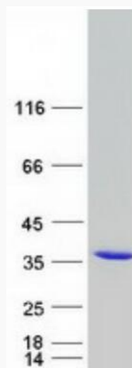
Coomassie blue staining of purified PEF1 protein.
