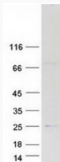
Coomassie blue staining of purified APOBEC3C protein.
