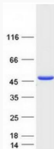
Coomassie blue staining of purified SERPINB4 protein.
