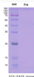
SDS-PAGE Image
