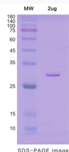
SDS-PAGE Image
