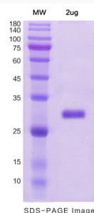
SDS-PAGE Image
