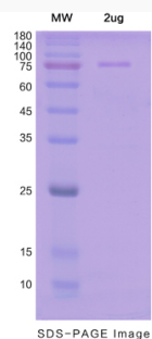
SDS-PAGE Image
