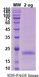
SDS-PAGE Image
