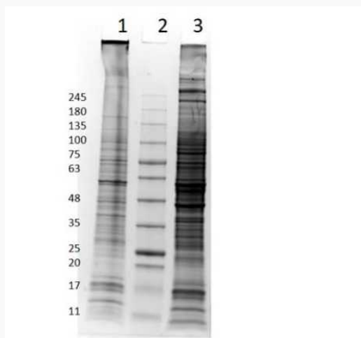
SDS-PAGE Results of A-172 Whole Cell Lysate. Lane 1: A-172 Whole Cell Lysate Non-Reduced [10 µg]. Lane 2: Opal Prestained Molecular Weight Marker. Lane 3: A-172 Whole Cell Lysate Reduced [10 µg]. 4-20% gel, coomassie stained.
