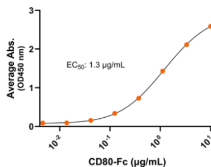
Mouse CD80-Fc dimer / CD28-His dimer ELISA 0.2µg of CD28 protein dimer per well
